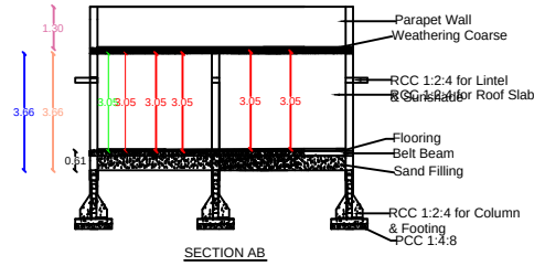
SECTION AB
