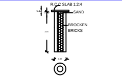
PERCOLATION PIT
