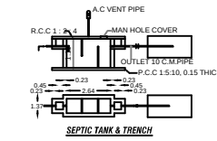
SEPTIC TANK & TRENCH
