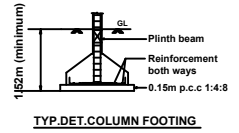
TYP.DET.COLUMN FOOTING
