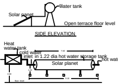
SOLAR WATER HEATER PLANT
