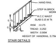
STAIR DETAILS
