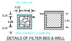
DETAILS OF FILTER BED & WELL
