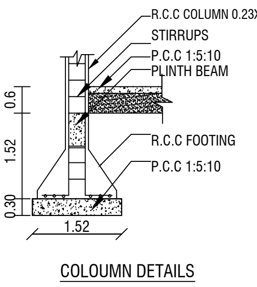
COLOUMN DETAILS
