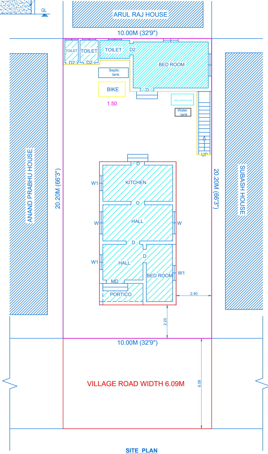
SITE PLAN
