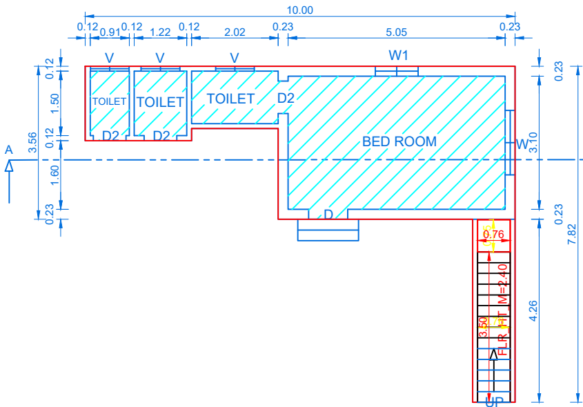
EXS.GROUND FLOOR PLAN
