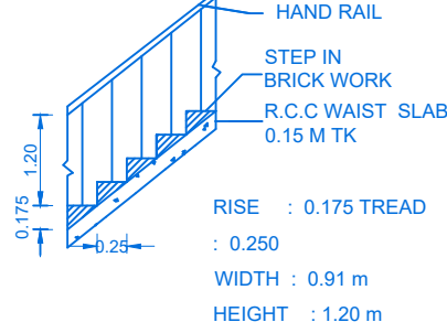
STAIR DETAILS
