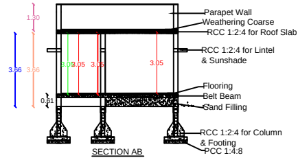
SECTION AB
