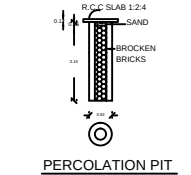
PERCOLATION PIT
