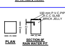
SECTION OF RAIN WATER PIT
