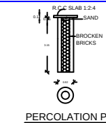
PERCOLATION PIT
