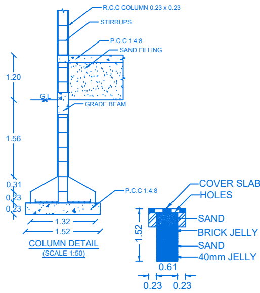
SECTION OF RAIN WATER COLLECTION TANK
