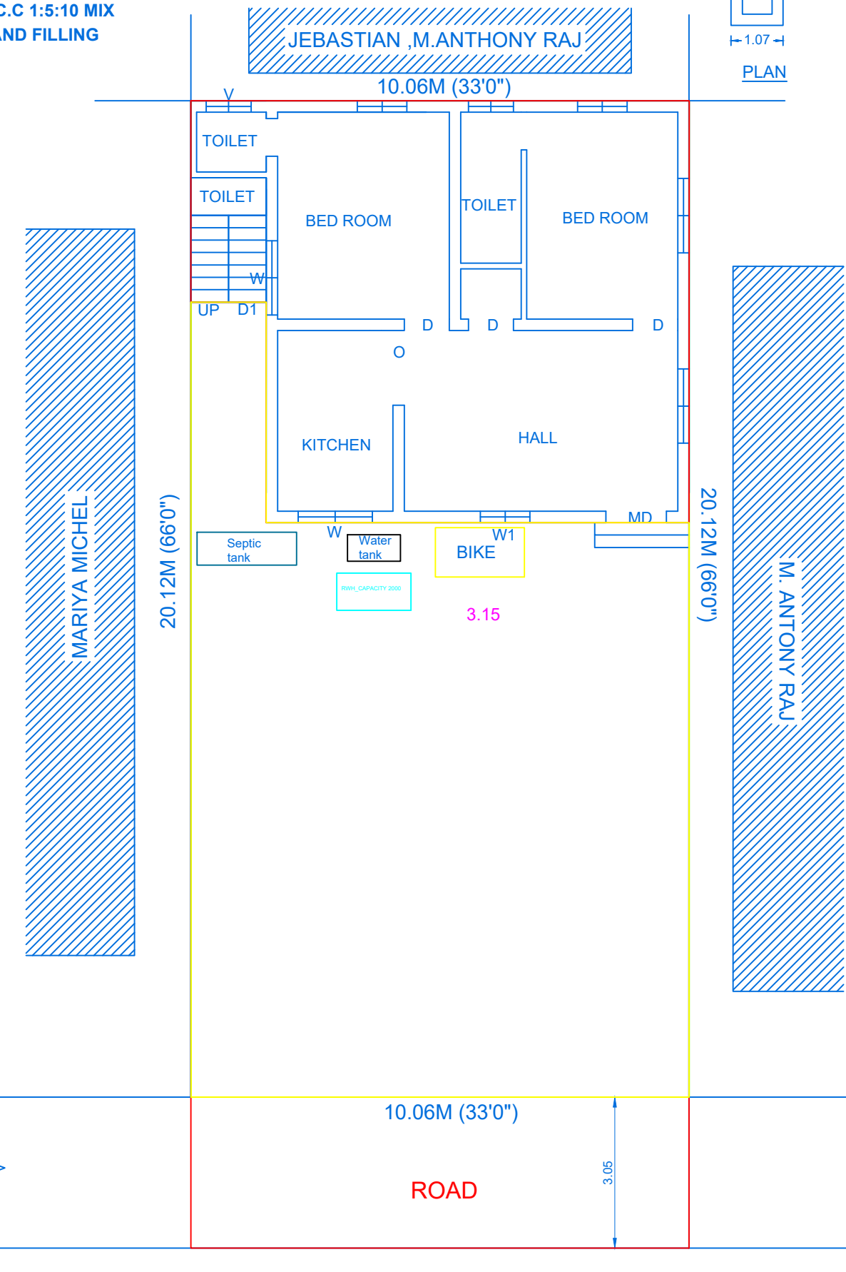
SITE PLAN
