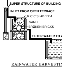
RAINWATER HARVESTING
