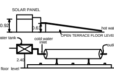
Details of solar water heating system
