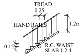
STAIRCASE DETAIL
