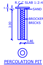
PERCOLATION PIT
