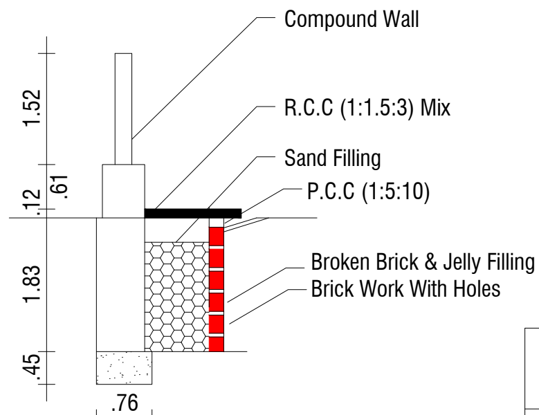
RAIN WATER HARVEST DETAILS
