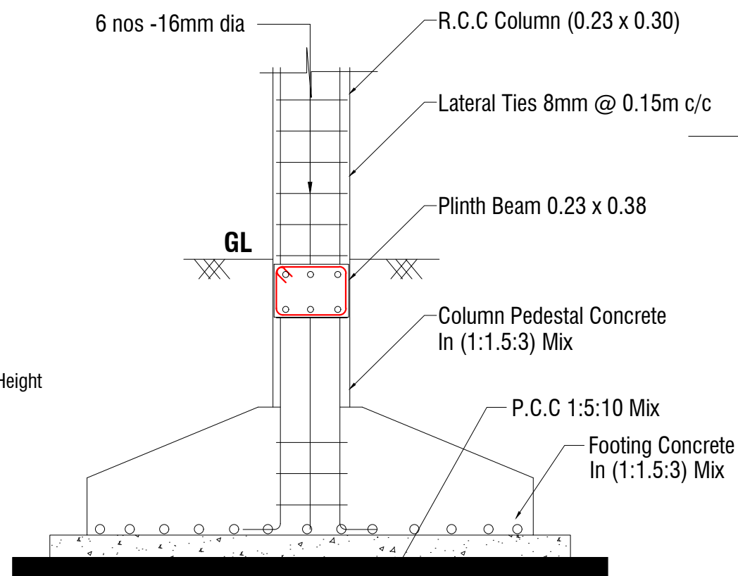
COLUMN FOOTING DETAILS
