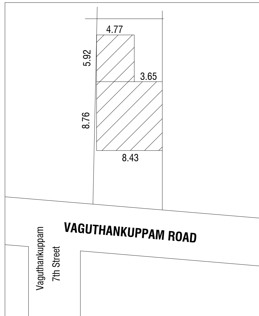
EXISTING BUILDING TO BE REMOVED
