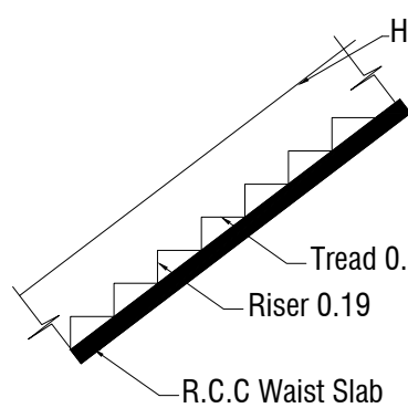
STAIR DETAILS
