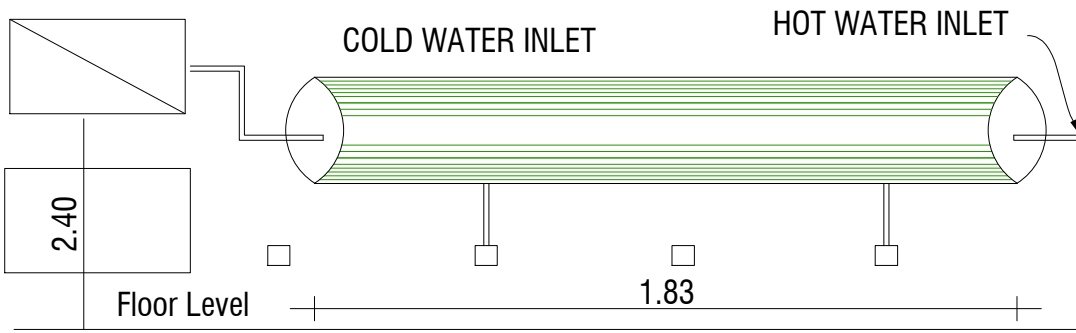
DETAILS OF SOLAR HOT WATER SYSTEM
