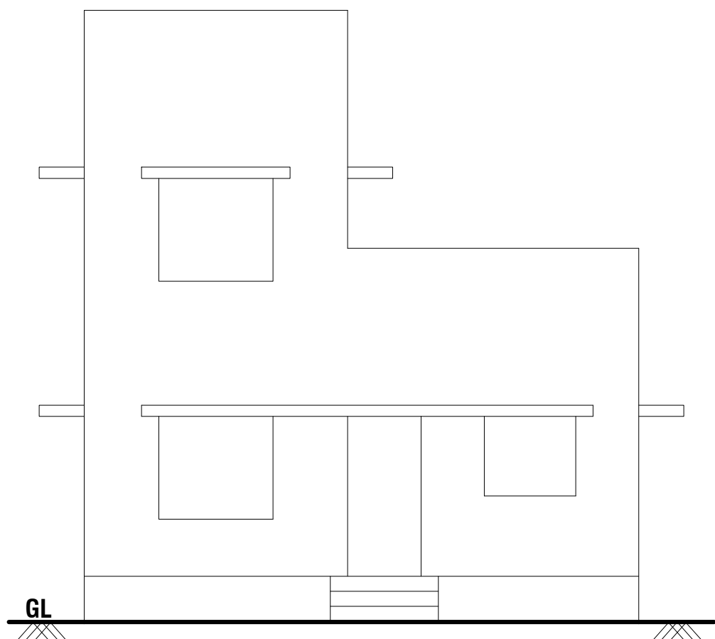
FRONT ELEVATION
