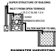
RAINWATER HARVESTING
