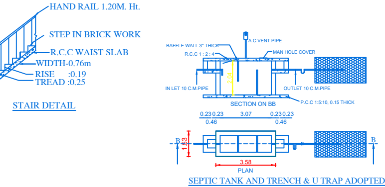
SEPTIC TANK AND TRENCH & U TRAP ADOPTED
