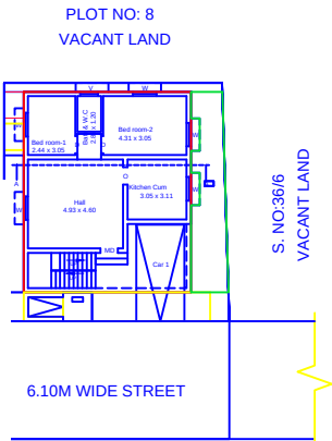
Floor Plan Scale 1:200
