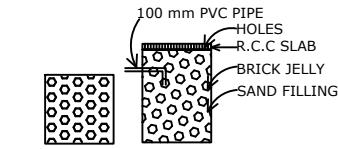
PLAN & SECTION OF RAINWATER COLLECTION TANK
