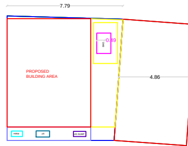
RESIDUARY PLOT SKETCH, SUPER IMPOSED (SITE PLAN)
