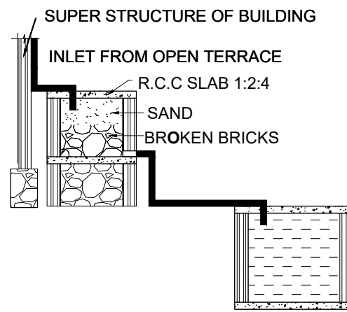
RAINWATER HARVESTING
