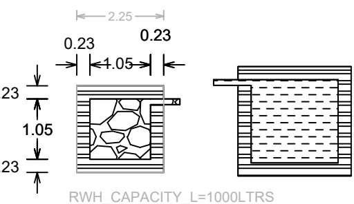
DETAILS OF FILTER BED & WELL
