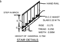
STAIR DETAILS
