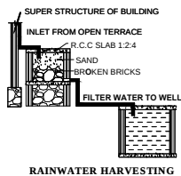
RAINWATER HARVESTING
