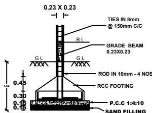
RCC COLUMN DETAILS
