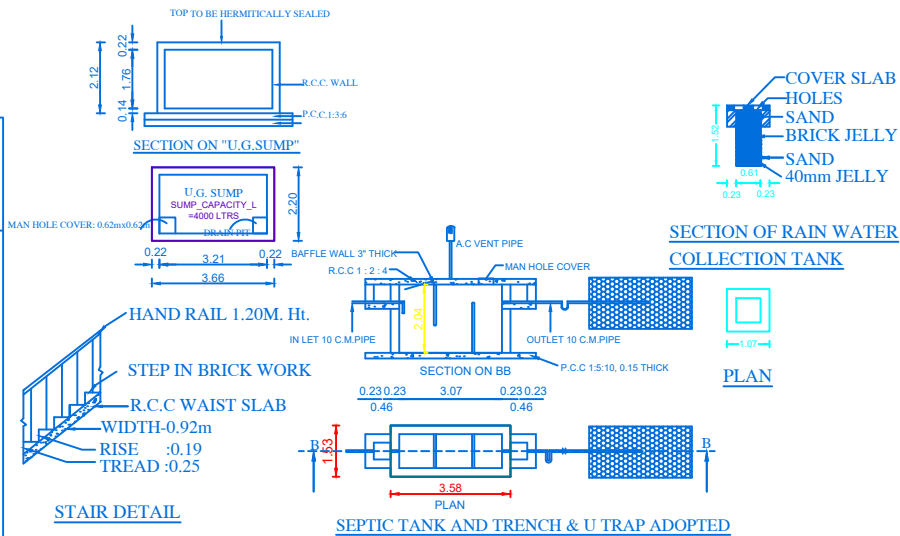
SEPTIC TANK AND TRENCH & U TRAP ADOPTED
