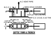
SEPTIC TANK & TRENCH
