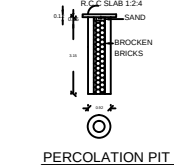
PERCOLATION PIT
