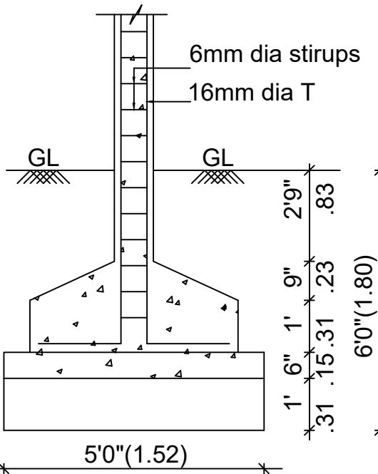
COLUMN FOUNDATION DETAIL
