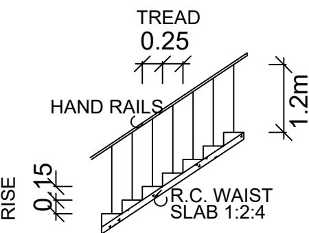
STAIRCASE DETAILS
