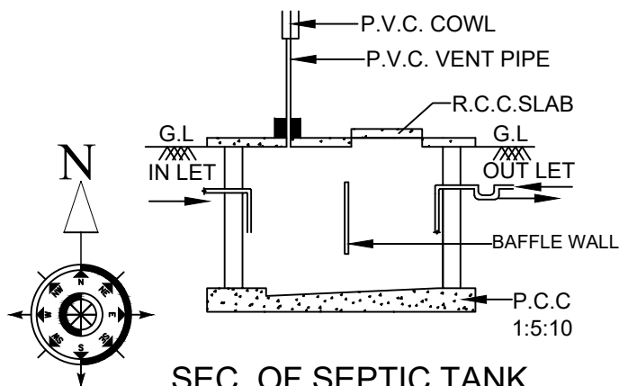
SEC. OF SEPTIC TANK
