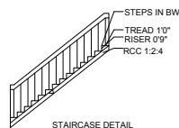
STAIRCASE DETAIL
