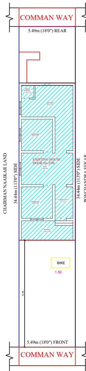
SITE PLAN
