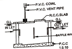
SEC. OF SEPTIC TANK
