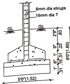
COLUMN FOUNDATION DETAIL
