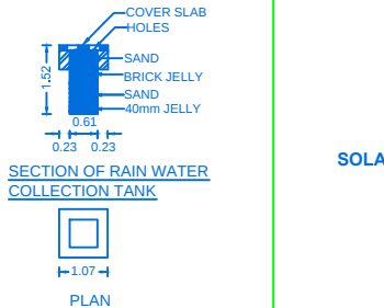
SECTION OF RAIN WATER COLLECTION TANK
