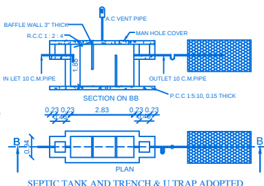
SECTION ON BB
