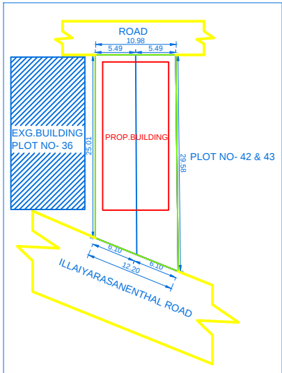
SITE PLAN (1:400 SCALE)
