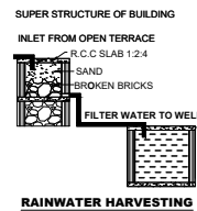
RAINWATER HARVESTING
