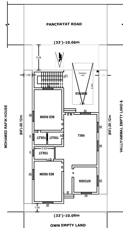
OWN EMPTY LAND SITE PLAN
