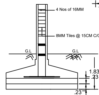
RCC COLUMN DETAILS
