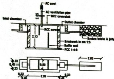
SEPTICTANK DETAILS
