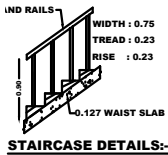
STAIRCASE DETAILS:-
