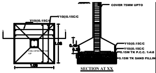
SECTION AT XX
