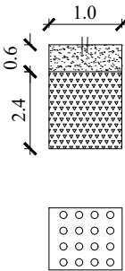
DETAIL OF RAIN WATER COLLECTING PIT- N.T.S
