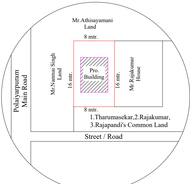
TOPO PLAN
