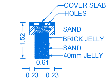
SECTION OF RAIN WATER COLLECTION TANK
