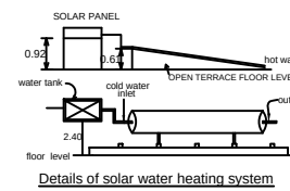
Details of solar water heating system
