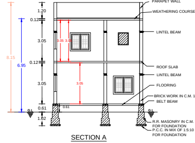
SECTION A
