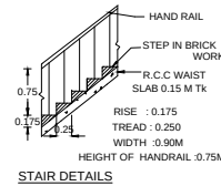
STAIR DETAILS
