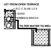
RAINWATER HARVESTING
