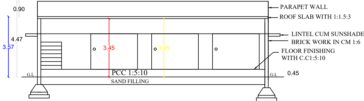
SECTION ON "A-B"
