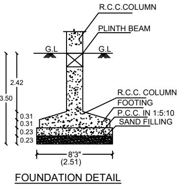
FOUNDATION DETAIL
