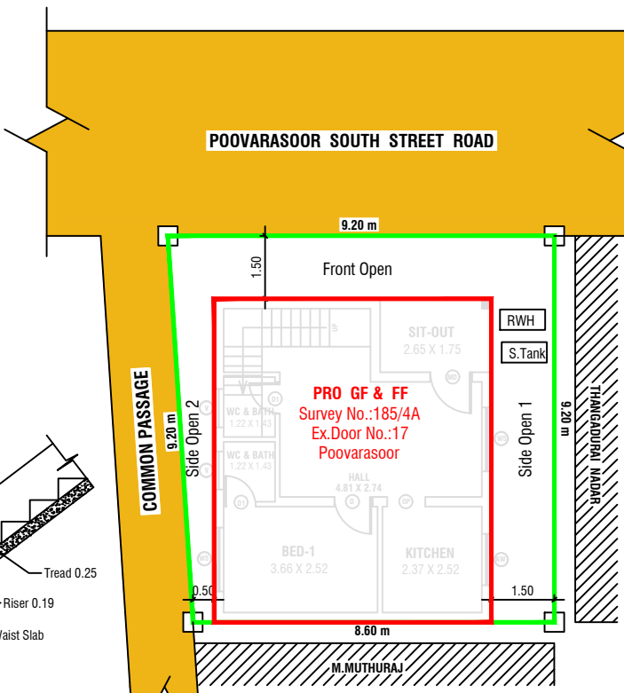
SITE PLAN (1:100)
