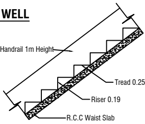
STAIR DETAILS
