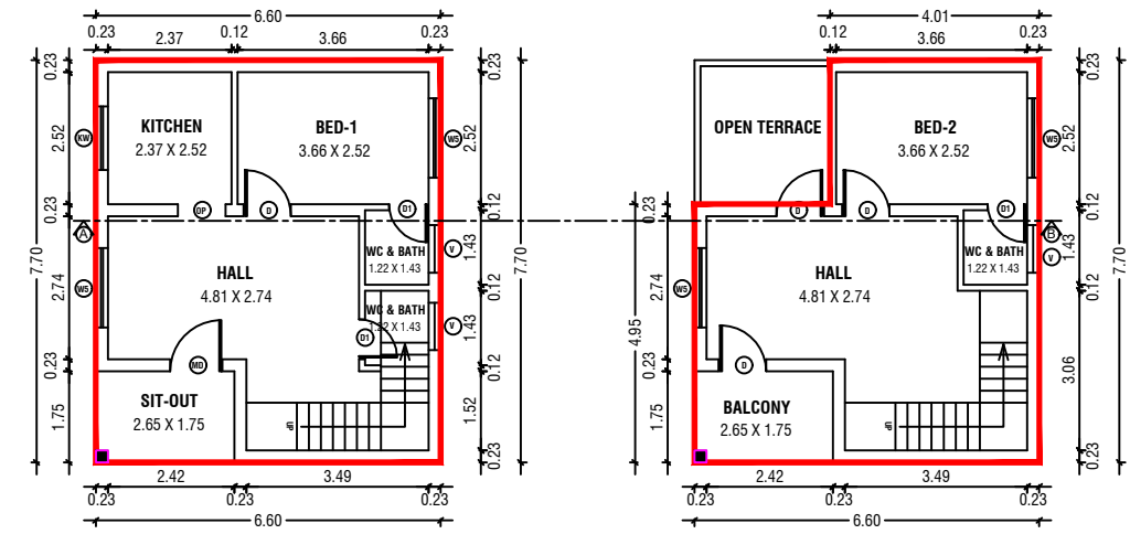
RAIN WATER HARVEST DETAILS
