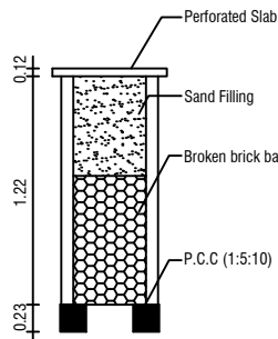
RAIN WATER HARVEST DETAILS
