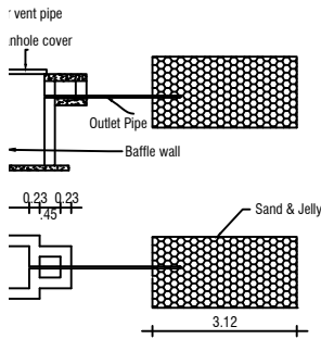
SEPTIC TANK & TRENCH
