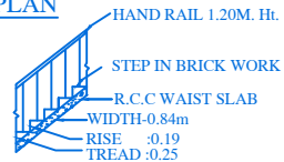
STAIR DETAIL
