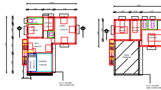
EXT. G.FLOOR PLAN
