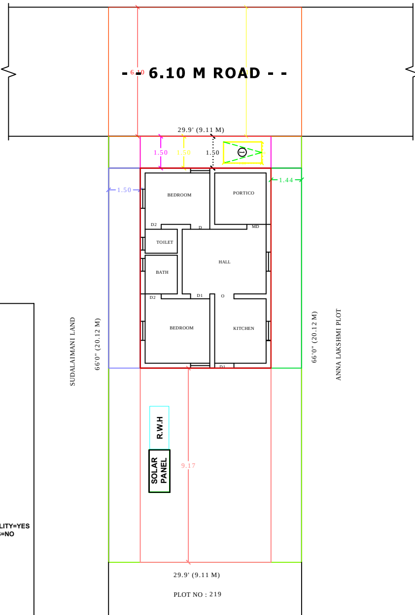
KEY PLAN
