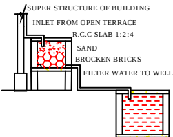
DETAILS OF FILTER BED & WELL
