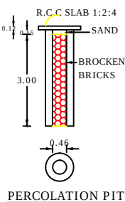
PERCOLATION PIT
