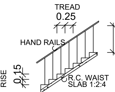
STAIRCASE DETAILS
