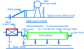
SOLAR WATER HEATER PLANT
