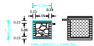
DETAILS OF FILTER BED & WELL
