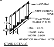
STAIR DETAILS
