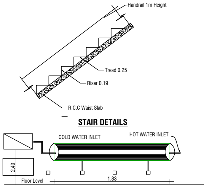
DETAILS OF SOLAR HOT WATER SYSTEM
