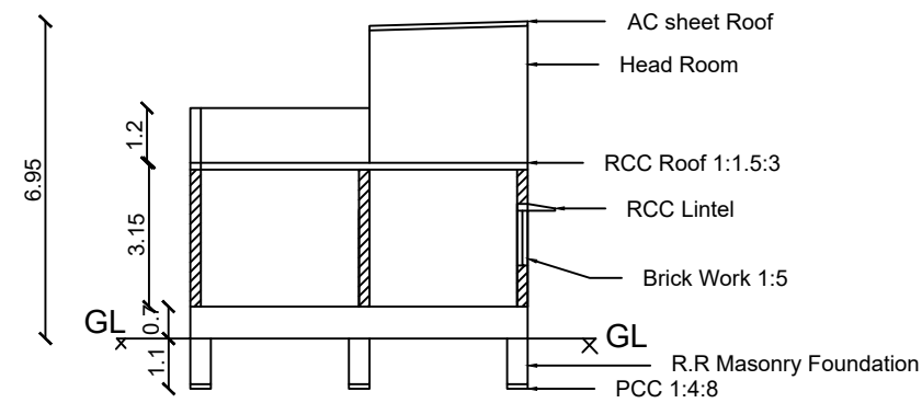
SECTION A-A VIEW
