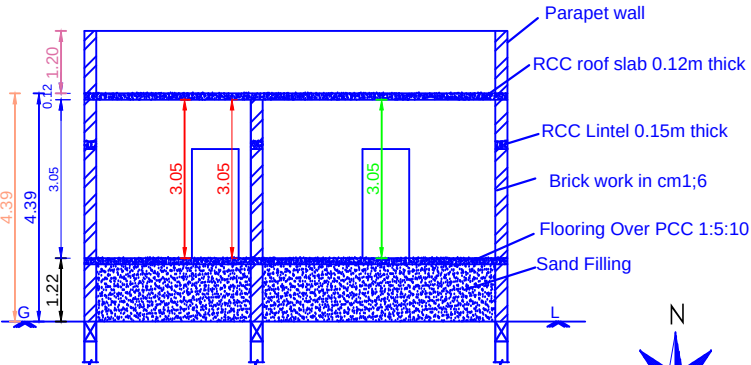
SECTION ON 'V-B'
