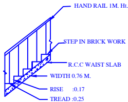
STAIR DETAIL
