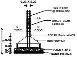
RCC COLUMN DETAILS
