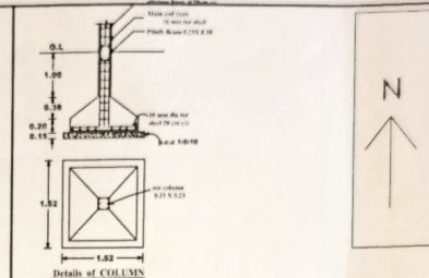
Details of COLUMN
