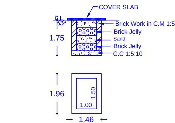
PLAN & SECTIONAL ELEVATION OF RAIN WATER HARVESTING
