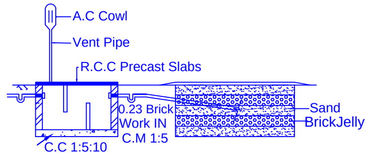
SECTION ON"BB" 'U' TROP MODEL S.T.ADOPTED )
