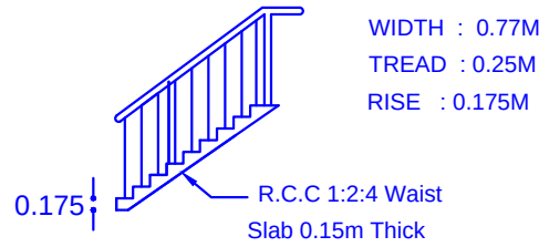
STAIRCASE SECTION
