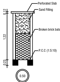
RAIN WATER COLLECTION WELL
