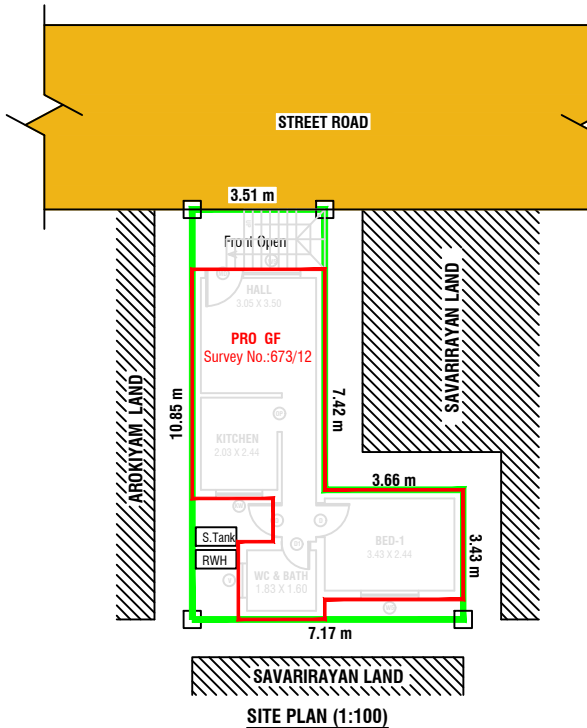
SITE PLAN (1:100)
