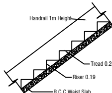
STAIR DETAILS
