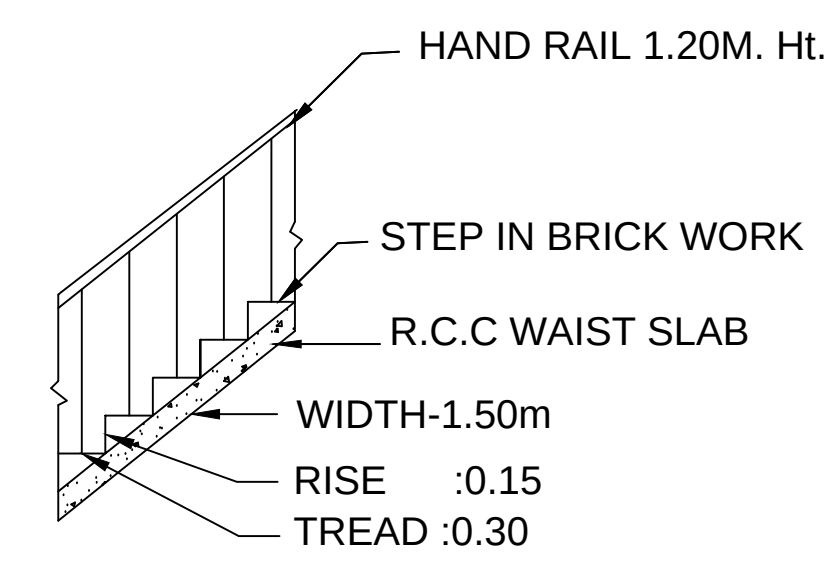
STAIR DETAIL
