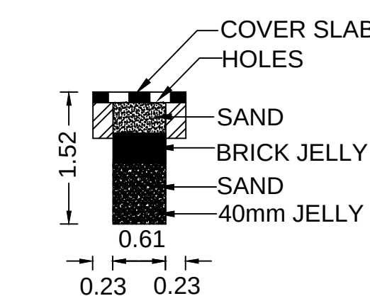
SECTION OF RAIN WATER COLLECTION TANK
