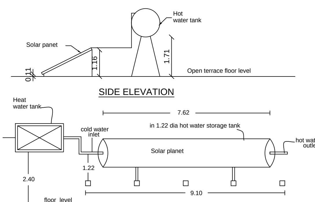
SOLAR WATER HEATER PLANT
