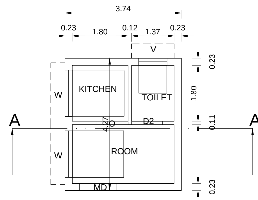
FLOOR PLAN
